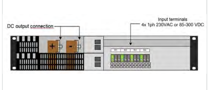
REAR VIEW FLATPACK 2 INTEGRATED 19" 2U
